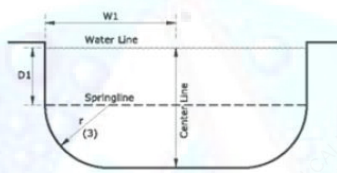
Figure 31B-3 Depths and Clearances for Pools without Diving Boards
